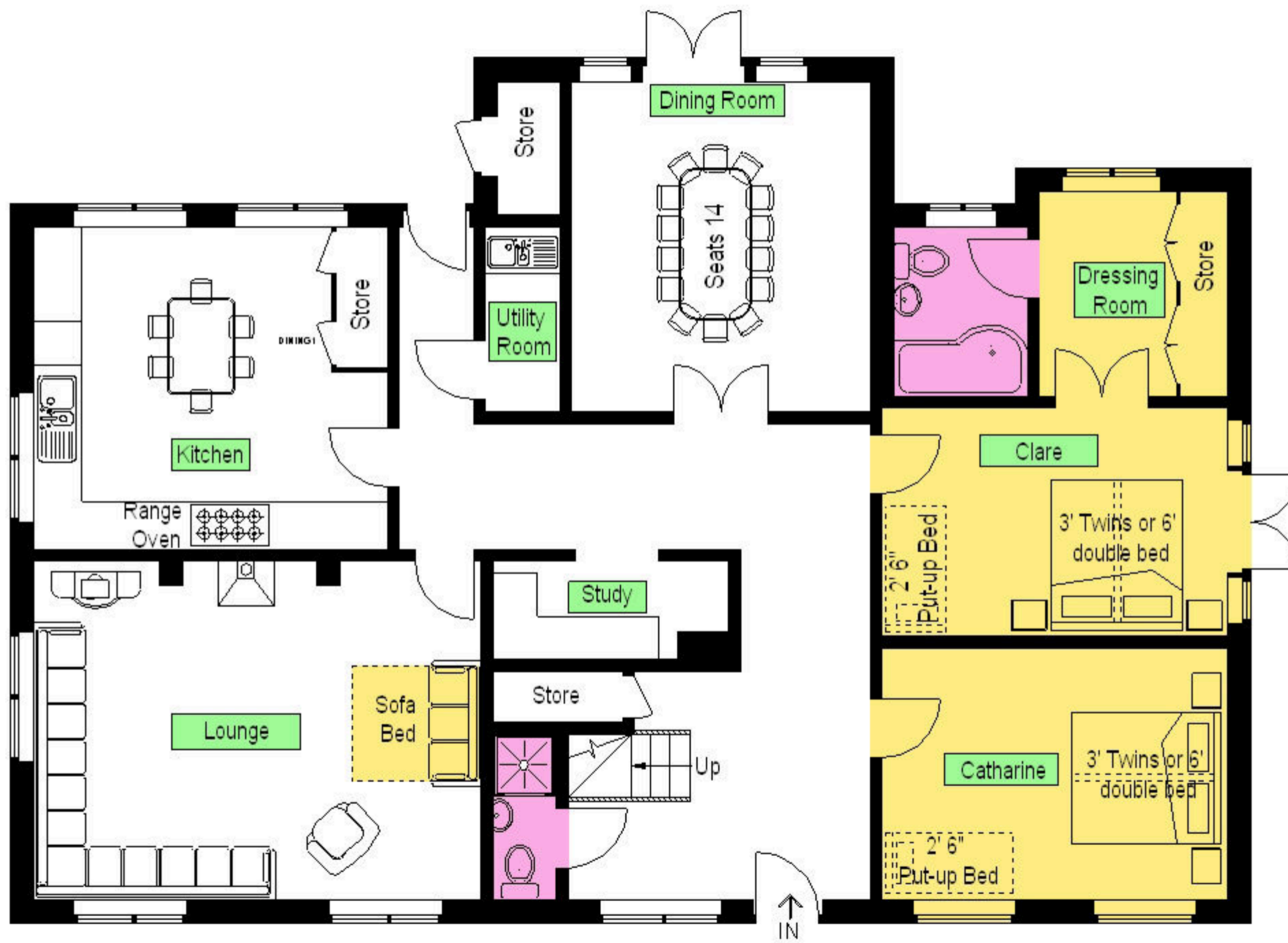
Ground Floor
